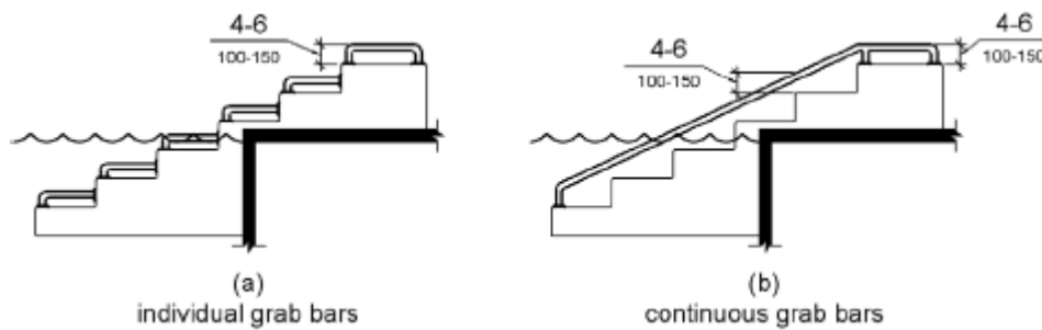
Figure 1009.5.7 Grab Bars
