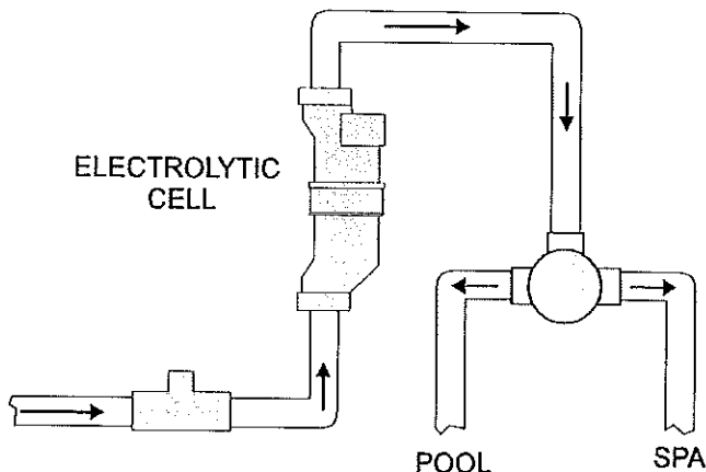
Vertical Installation
